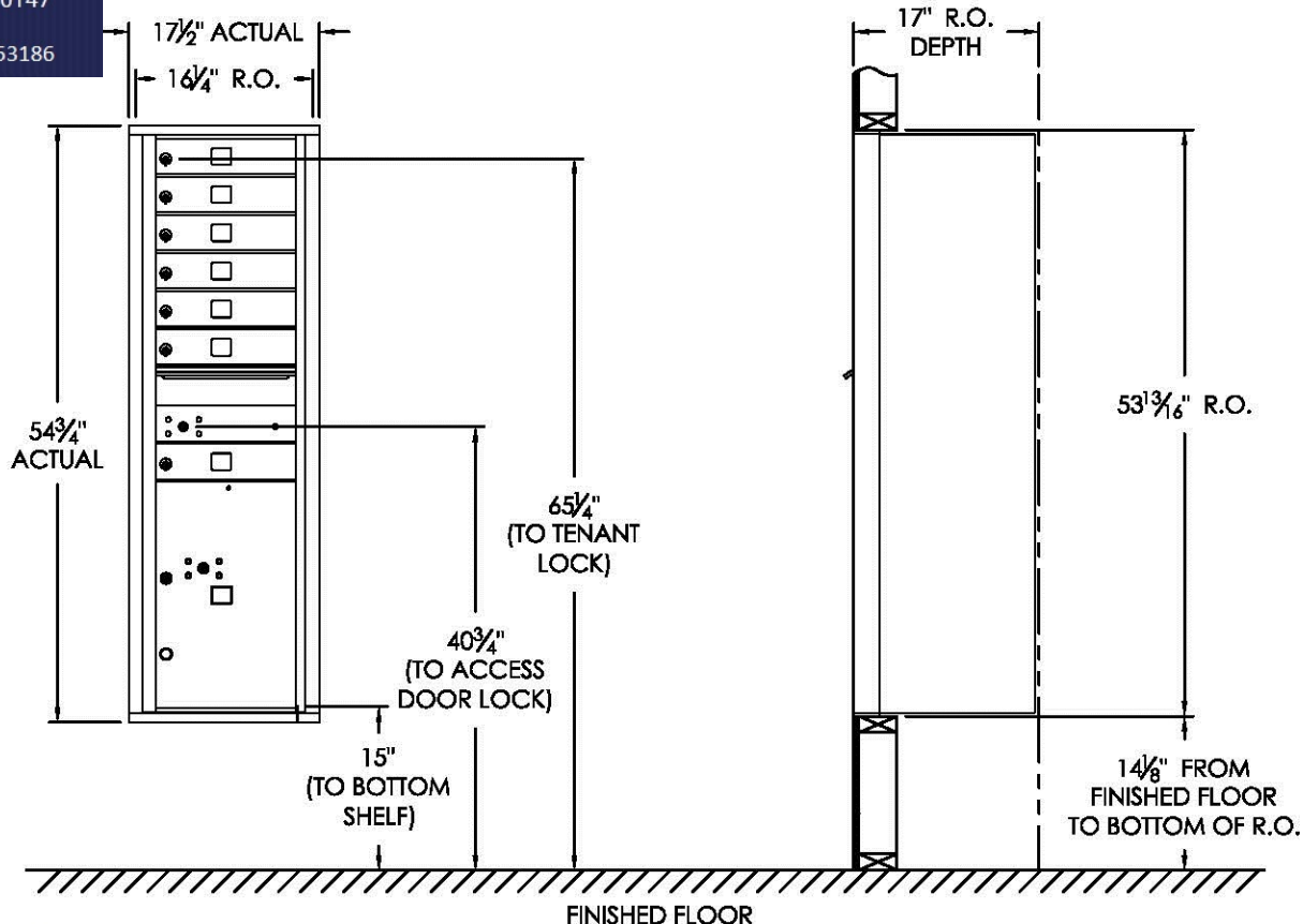
COMPARTMENT CHART
