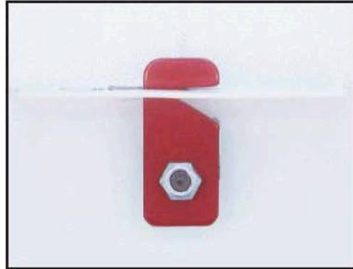
"Hook" cam engaged in box frame
