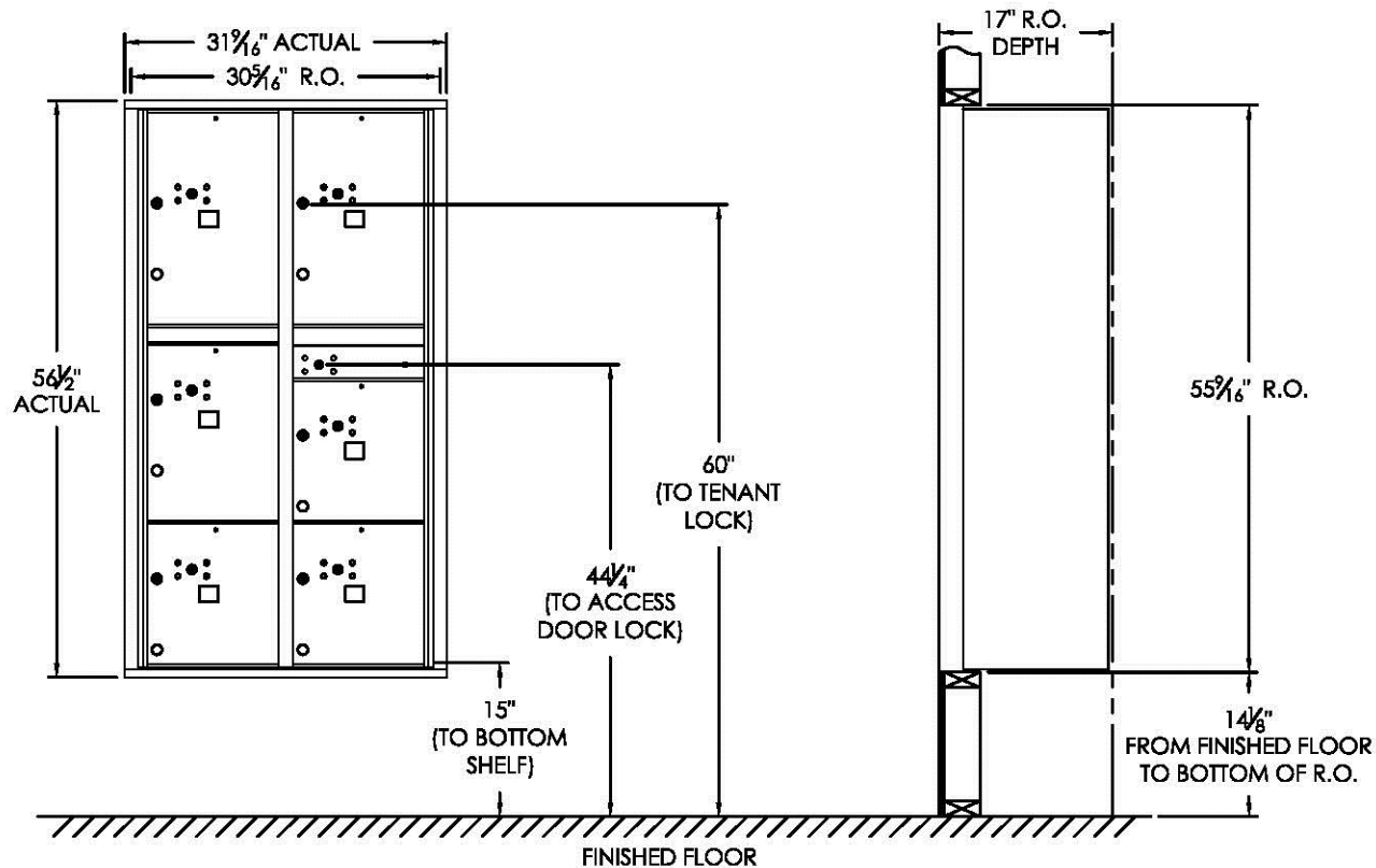
COMPARTMENT CHART
